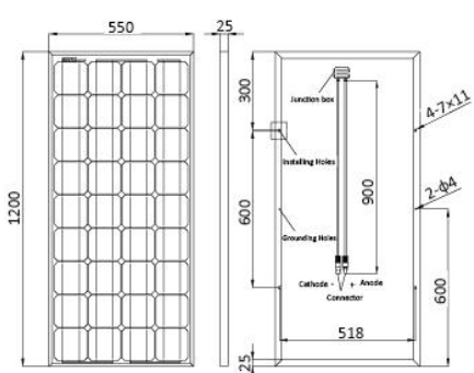
GSM-100W-M
